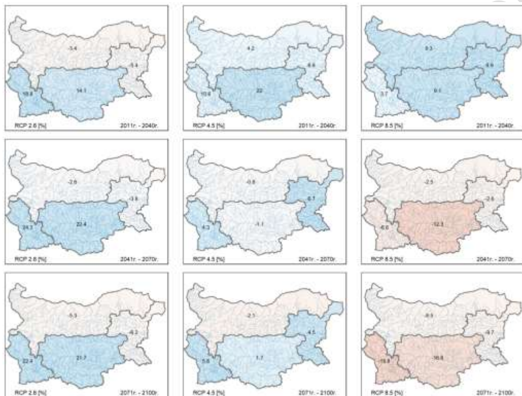
Fig. 2. Maps of relative change of the multiannual average runoff in the four main river basin districts, for the three 30 year periods 2011-2040, 2041-2070 and 2071-2100 in [%] compared to the reference 2071 – 2000. At the left – relative change for RCP 2.6; in the middle – for RCP 4.5 and to the right for RCP 8.5.
