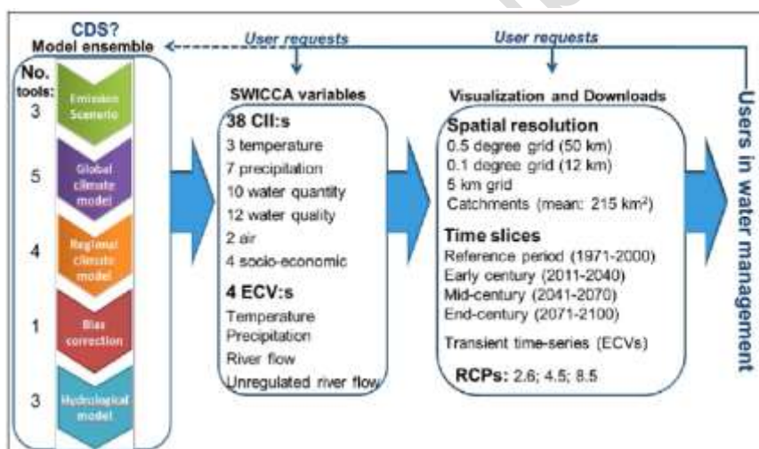
Fig. 1. Production tool-chain for about 900 data sets in SWICCA demonstrator (Nov. 2016).
